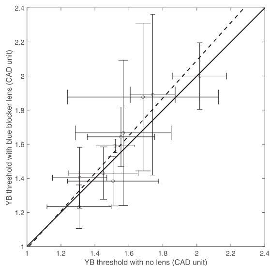
Fig. 7. – Relationship between the YB threshold with no lens ( x -axis) and with blue blocker lens ( y -axis). The error bars are the standard deviations. The dashed line is the regression line ( y = 1.10x - 0.11 ), the solid line is the y = x line. Pearson's r = 0.92 .
